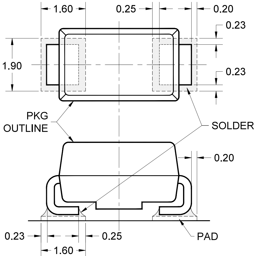
PAD LAYOUT
