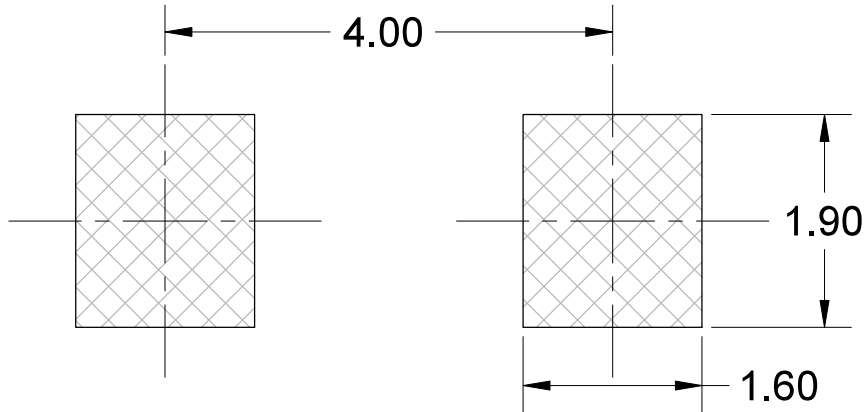
PAD LAYOUT
